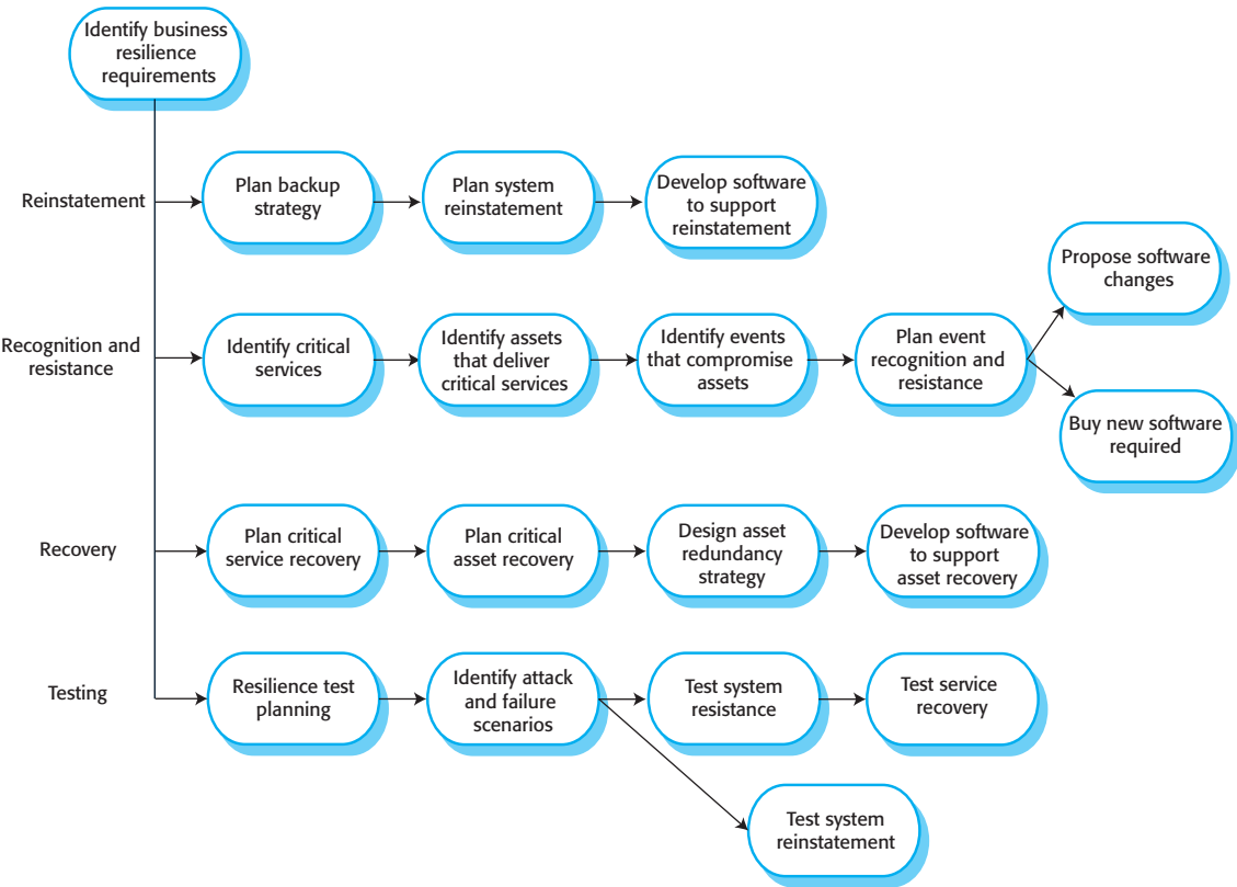
Figure 14.9 Resilience engineering
